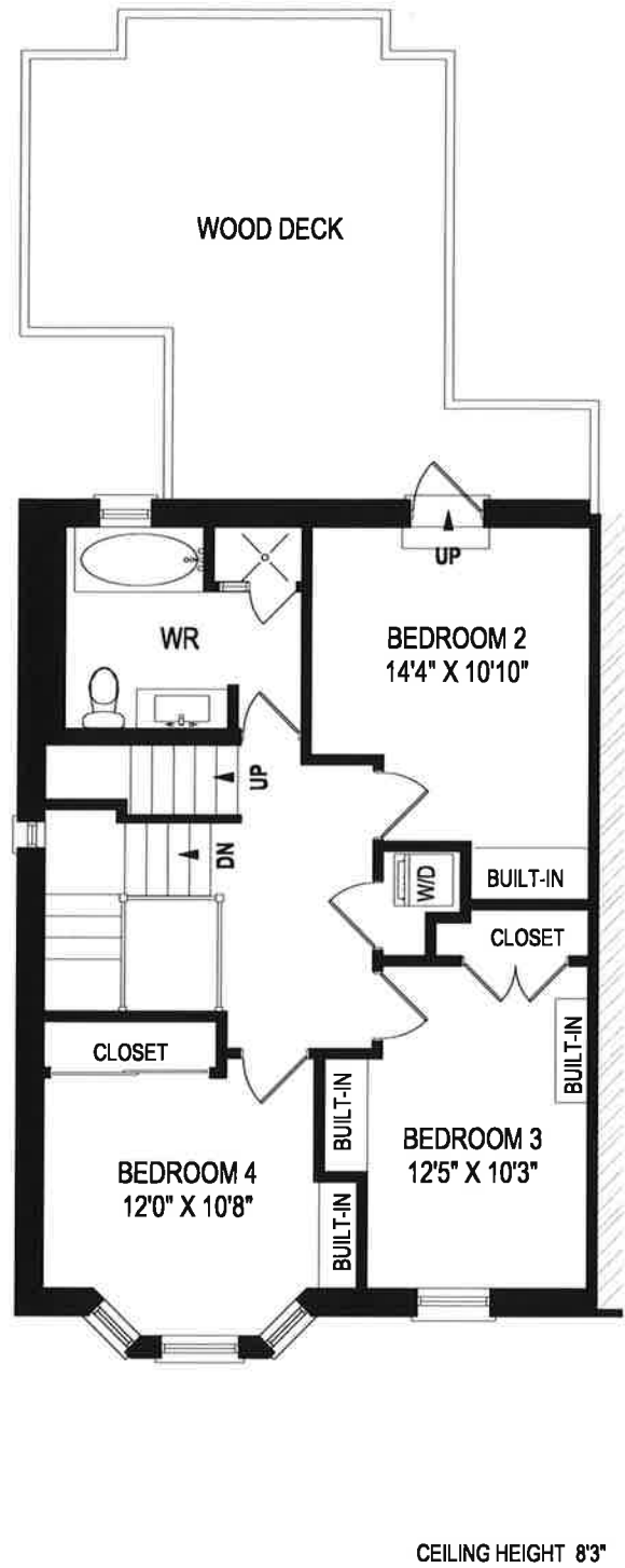
SECOND FLOOR - 725 SQUARE FEET
