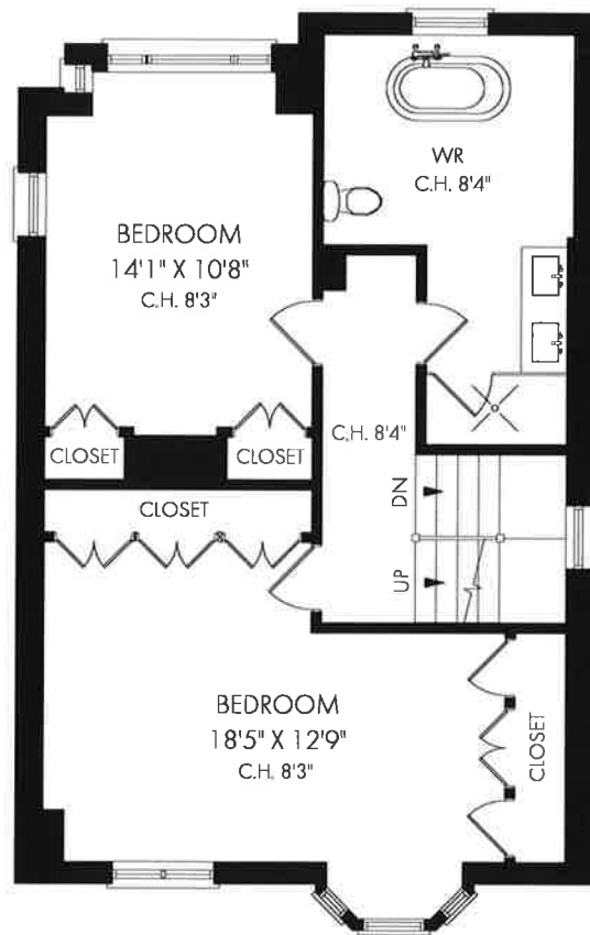
CEILING HEIGHT 8'4" SECOND FLOOR - 791 SQUARE FEET
